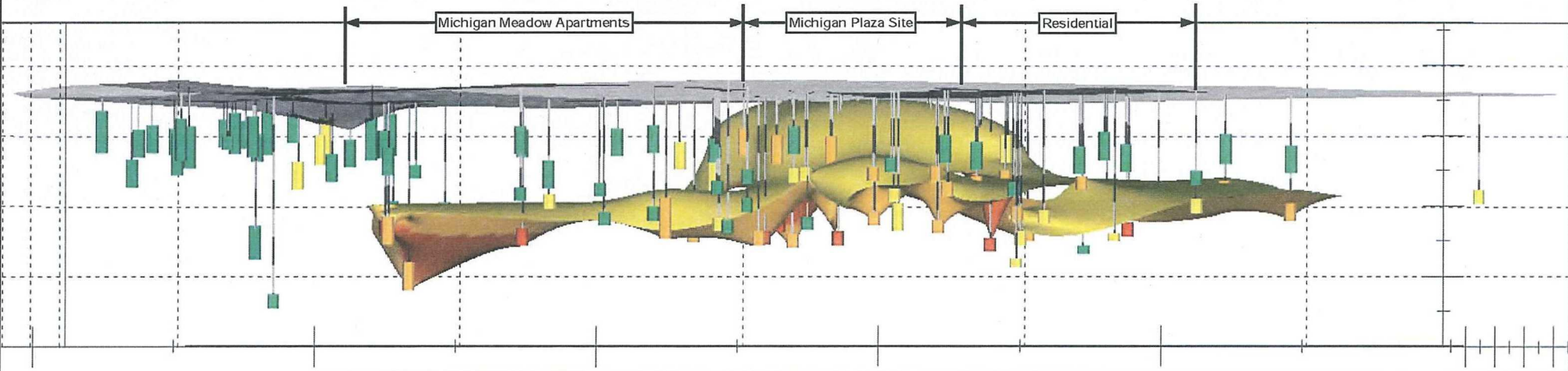
Figure 6 Vinyl Chloride (VC) Plume Above 20 µg/L
