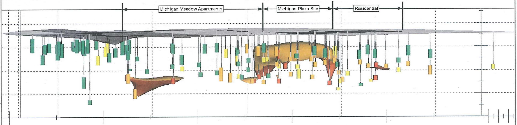
Figure 7 Vinyl Chloride (VC) Plume Above 200 µg/L
