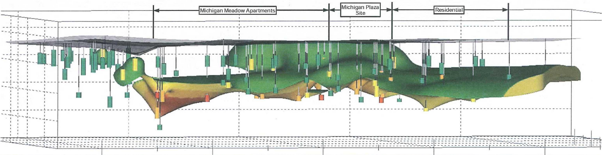
Figure 5 Vinyl Chloride (VC) Plume Above 2 µg/L
