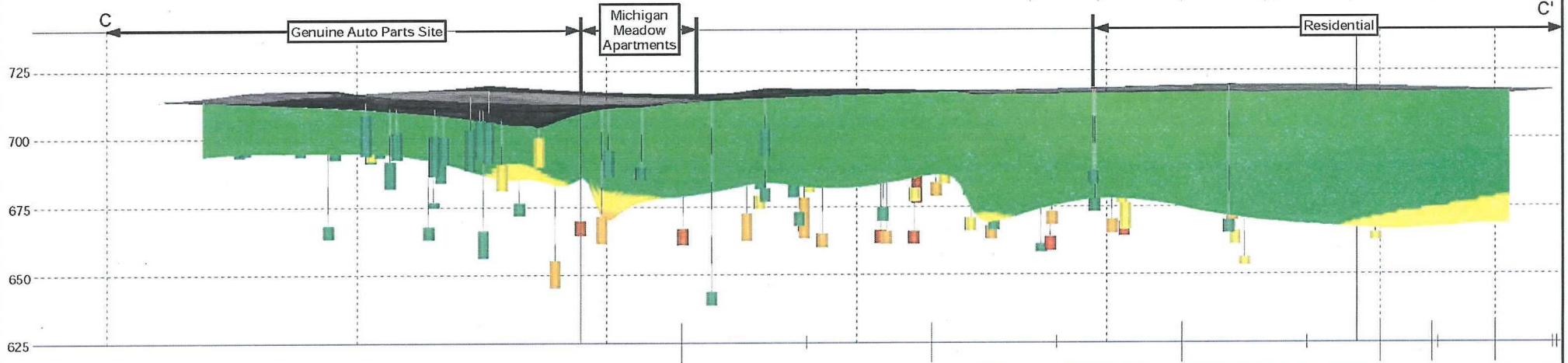
Figure 11 Cross Section C - C' Through Genuine Parts
