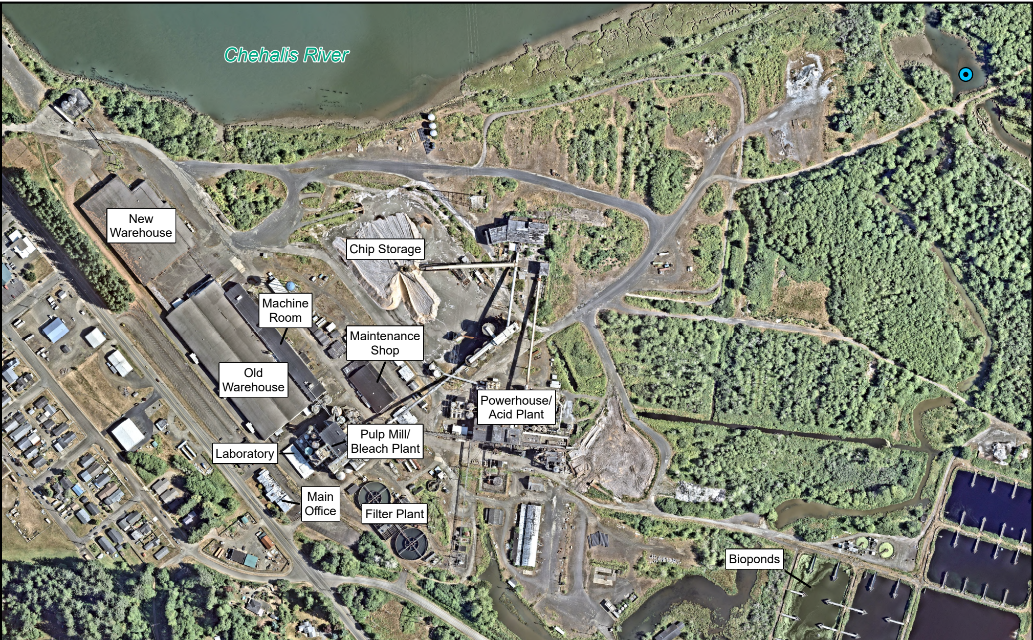
FIGURE 2 SITE FEATURES - MAIN FACILITY COSMO SPECIALTY FIBERS 2025 RSE COSMOPOLIS, WA February, 2026
