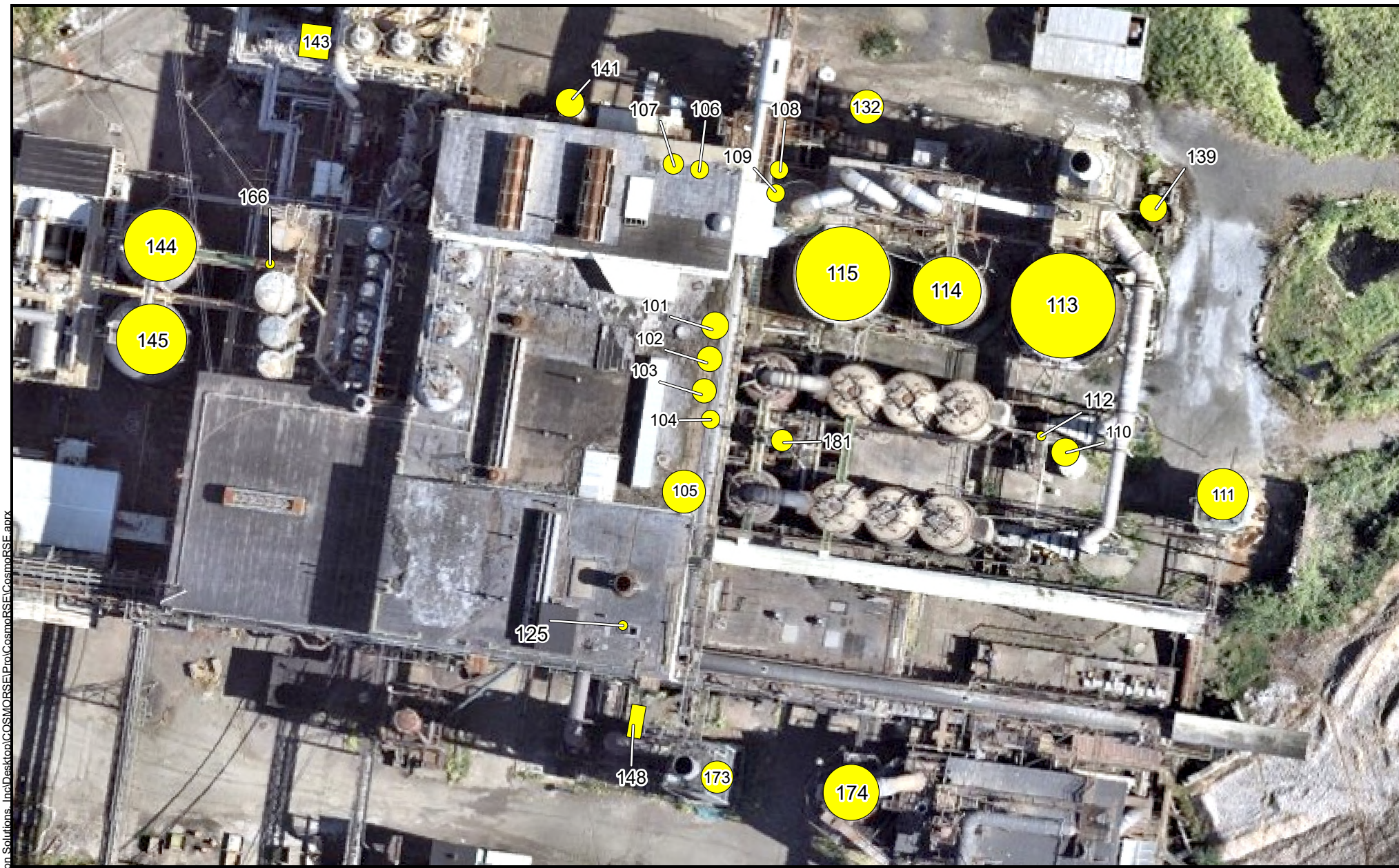
FIGURE 10 CERCLA HAZARDOUS SUBSTANCE TANKS POWERHOUSE COSMO SPECIALTY FIBERS 2025 RSE COSMOPOLIS, WA February 2026
