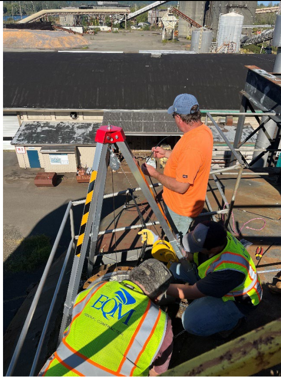
EPA contractors placing submersible pump inside Dump Tank 1.
